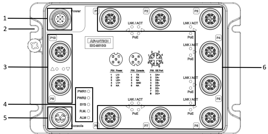
Figure 1.1 Front View
