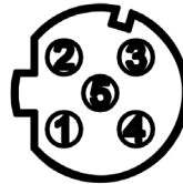
Figure 2.7 M12 D-Coded Connector Pin Assignment
