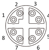
Figure 2.8 M12 X-Coded Connector Pin Assignment
