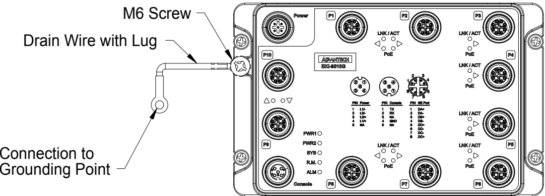
Figure 2.4 Grounding Connection, Chassis Left Side View
