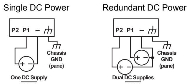
Figure 2.3 Power Wiring for EKI-9510 Series
