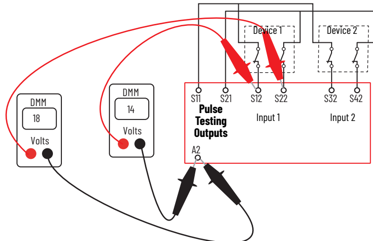
Figure 65 - Typical Voltage Measurements of the DI, DIS, and SI Safety Relays with Contacts Closed
