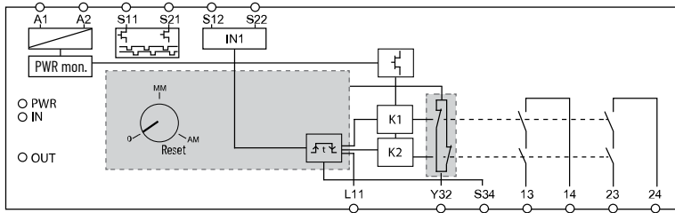
Figure 42 - SI Safety Relay Circuit Diagram
