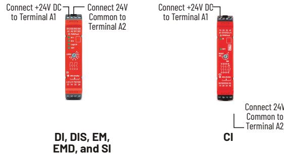
Figure 7 - Power Supply Connections
