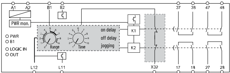
Figure 41 - EMD Safety Relay Circuit Diagram
