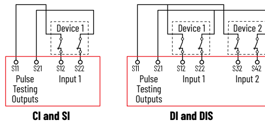
Figure 8 - Example Connections to 2 N.C. Mechanical Contacts
