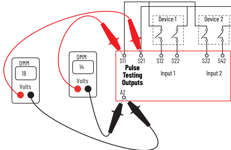
Figure 64 - Typical Voltage Measurements of the DI, DIS, and SI Safety Relays with Contacts Open
