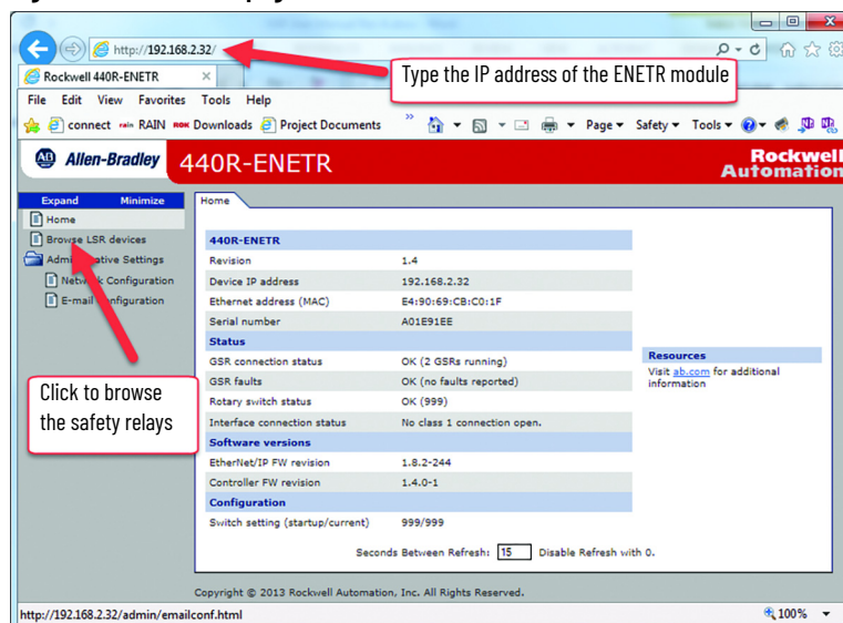
Figure 55 - ENETR Webpage
