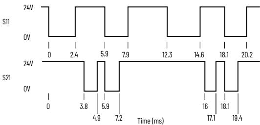
Figure 30 - Pulse Test Sequence for DI, DIS, and SI Safety Relays
