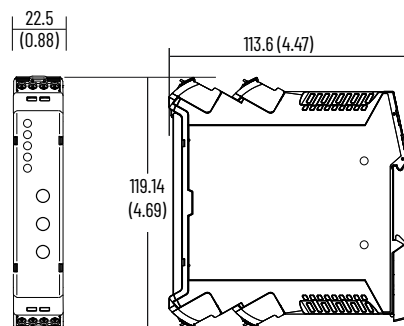
Figure 2 - Approximate Dimensions [mm (in.)]
