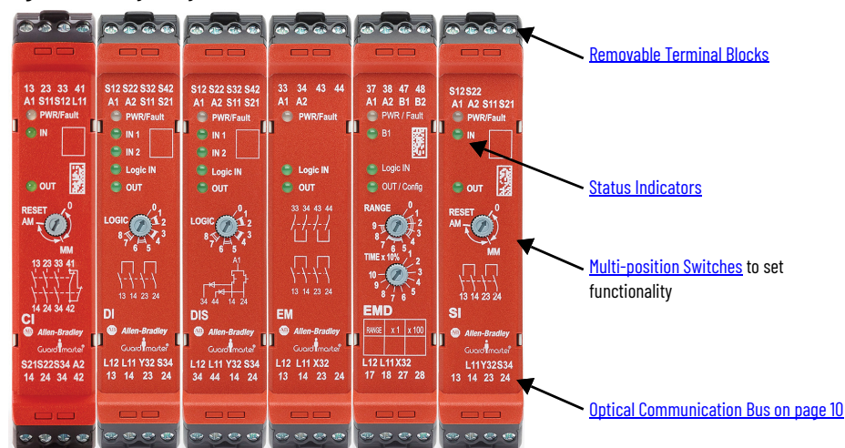
Figure 1 - Safety Relays
