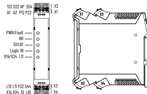
Figure 5 - Terminal Identification
