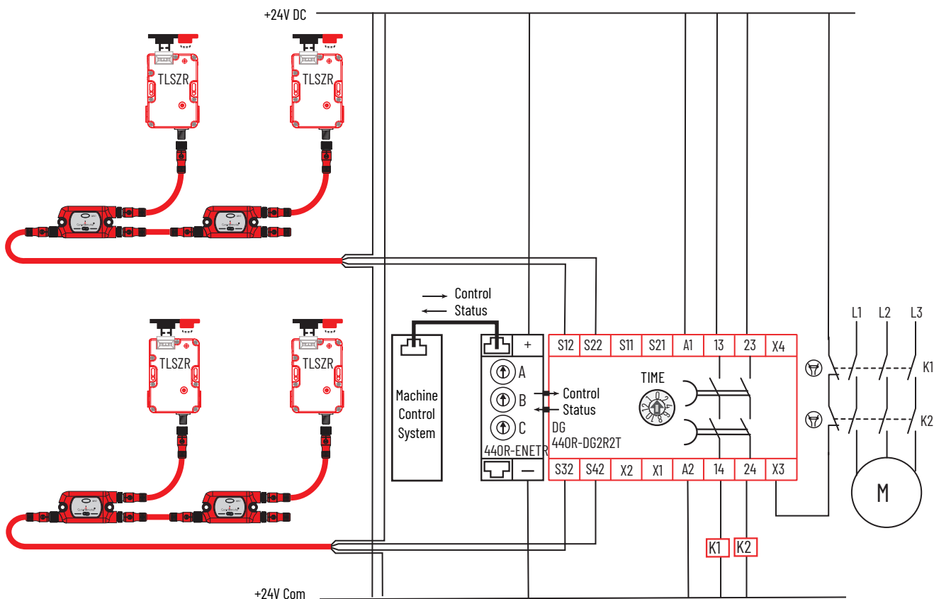
Figure 19 - DG with TLSZR Schematic
