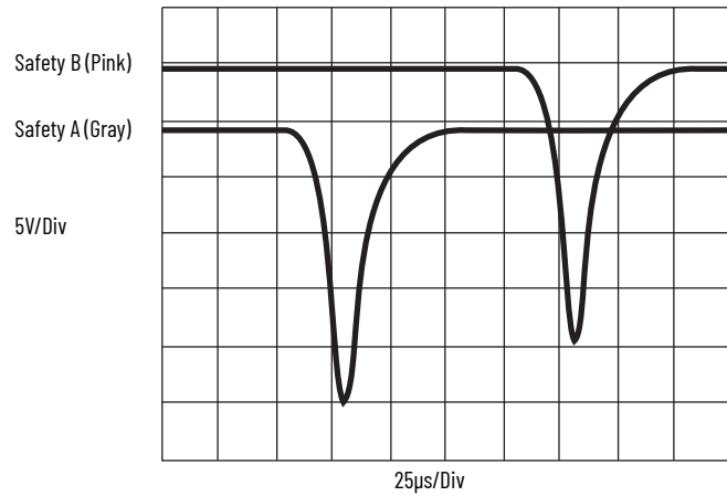
Figure 14 - Output Test Pulses
