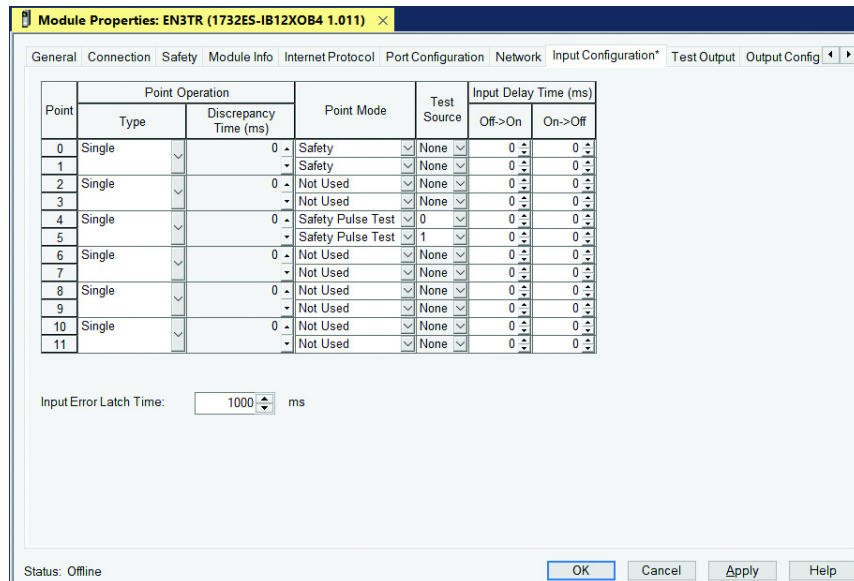
Figure 31 - Module Properties - Input Configuration
