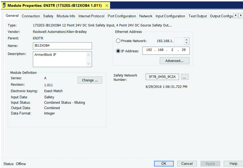
Figure 30 - Module Properties - General
