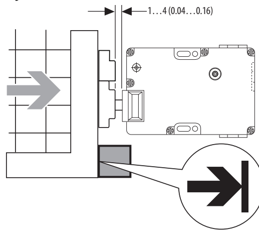
Figure 38 - Clearance in Closed Position [mm (in.)]
