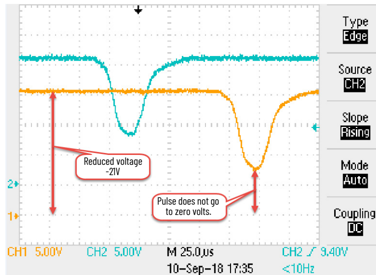
Figure 40 - Effect of 300 \Omega of Wire Resistance Going Into a GSR-SI Safety Relay
