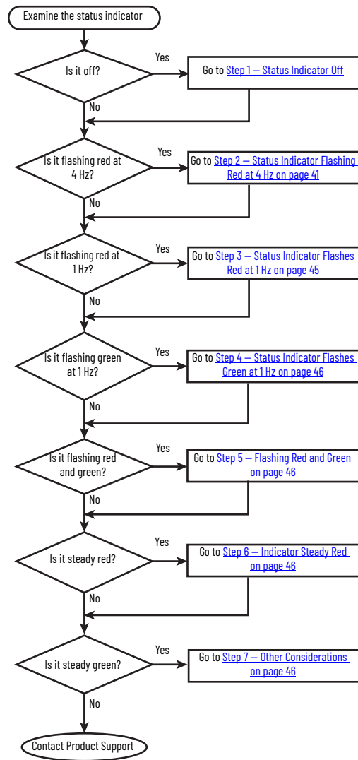
Figure 35 - Troubleshooting Flow Diagram
