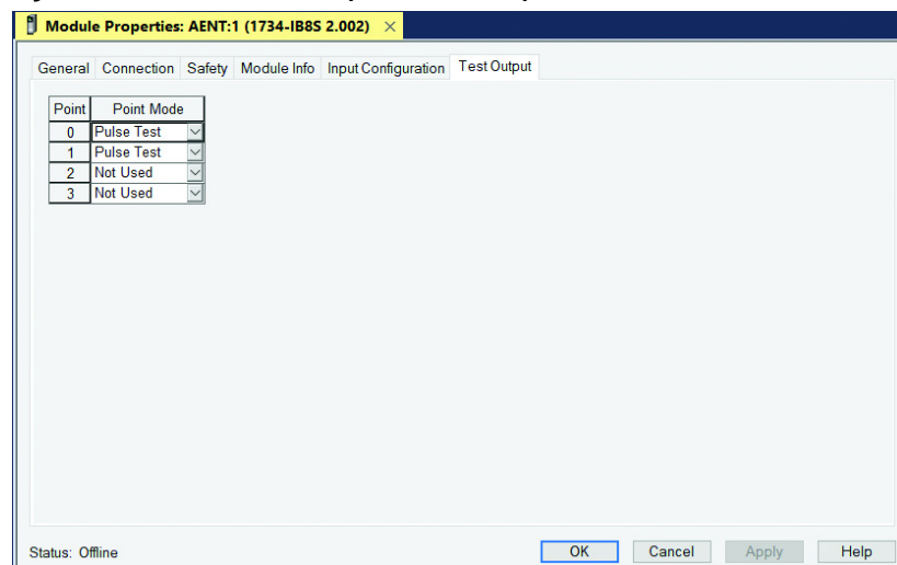
Figure 25 - 1734-IB8S Module Properties - Test Output
