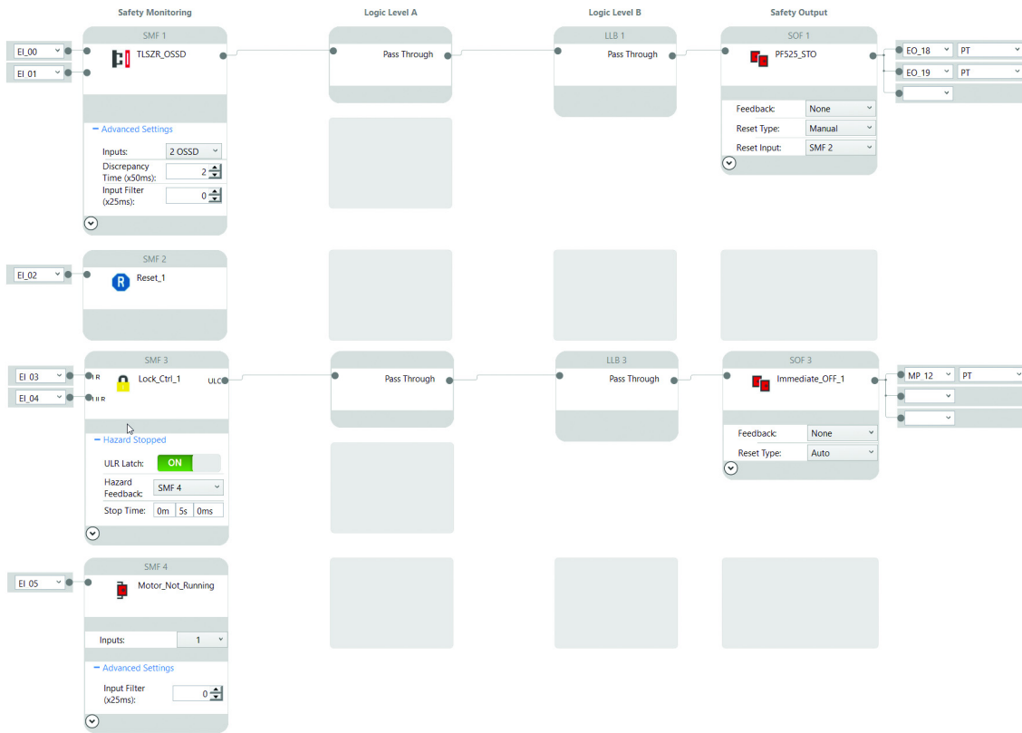
Figure 21 - CR30 Configuration in Connected Components Workbench
