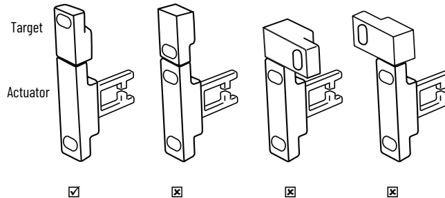
Figure 37 - Mounting of Target and Actuator
