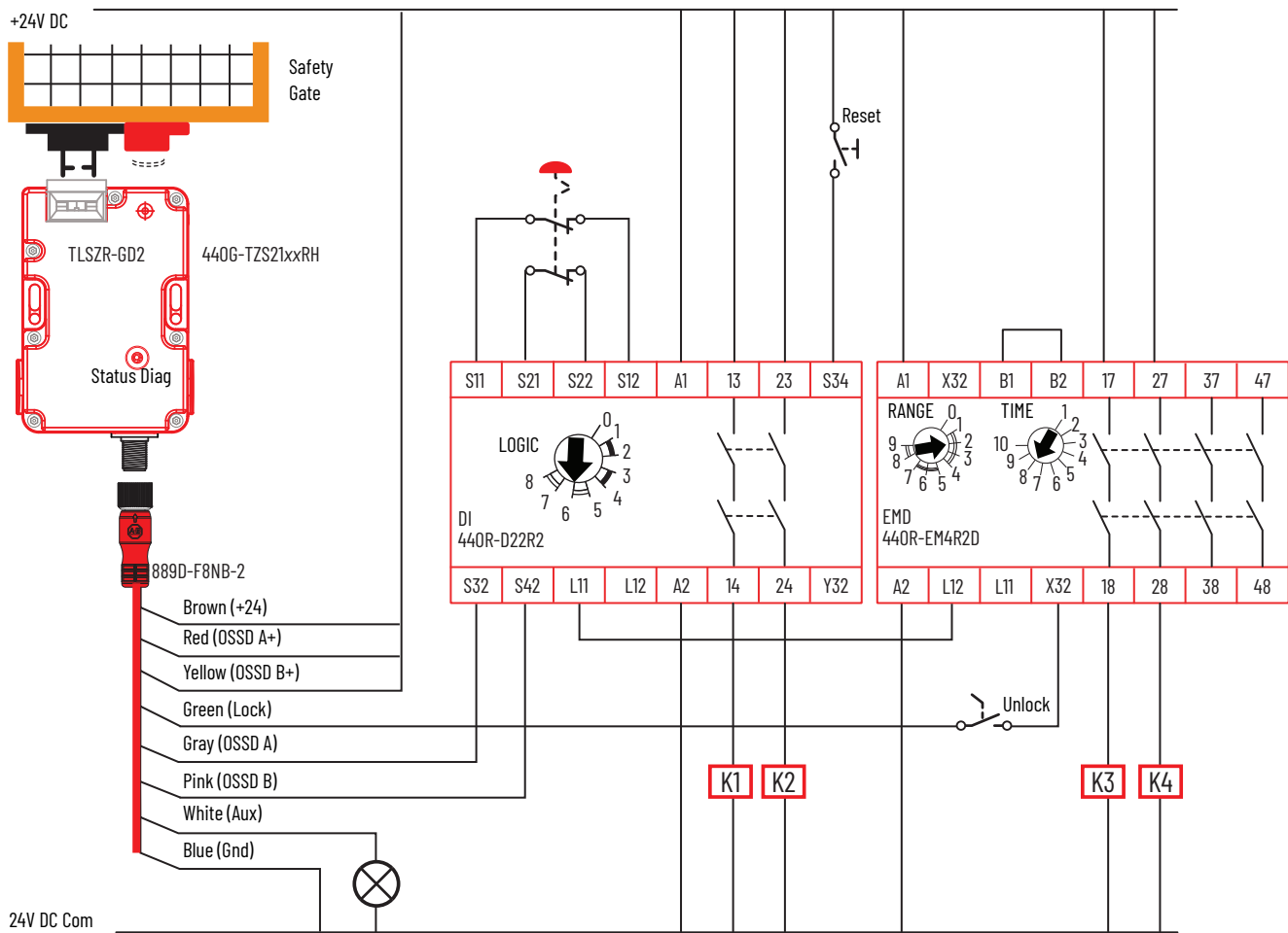
Figure 18 - DI with EMD and TLSZR Schematic
