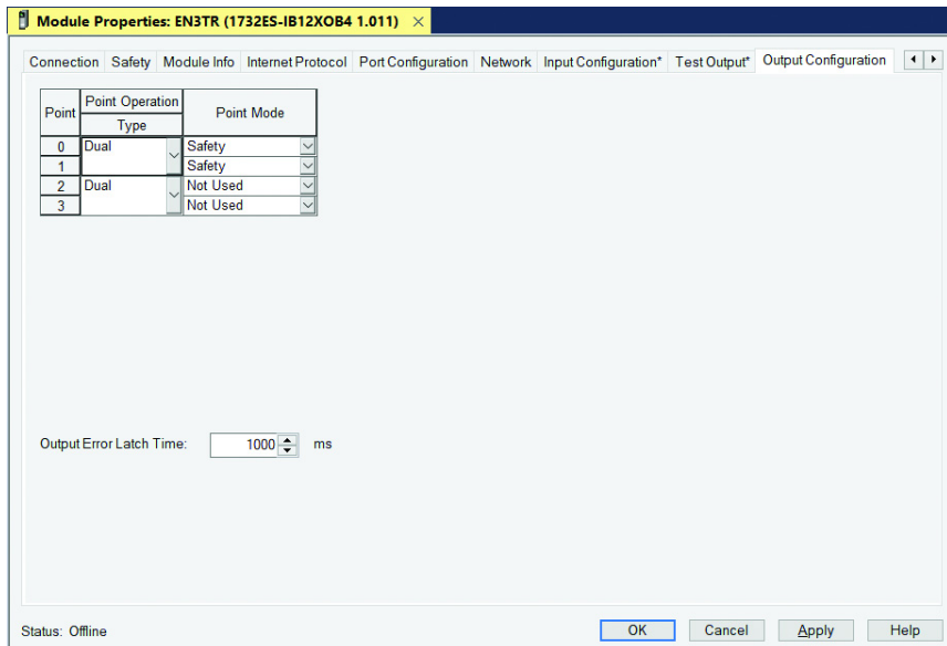
Figure 33 - Module Properties - Output Configuration
