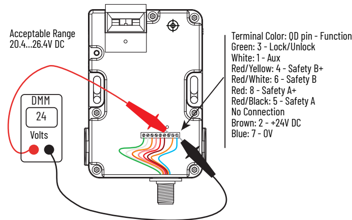
Figure 36 - Measure the Voltage at the Power Supply Terminals
