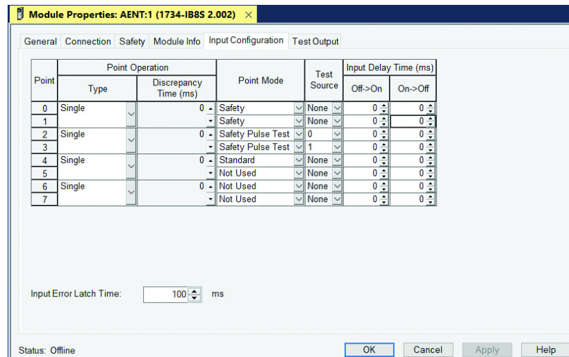
Figure 24 - 1734-IB8S Module Properties - Input Configuration
