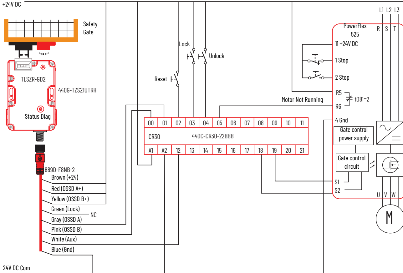
Figure 20 - CR30 Schematic
