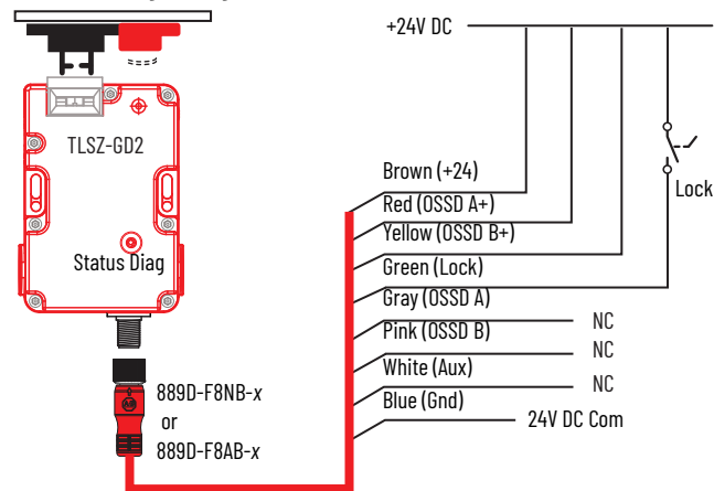
Figure 15 - Commissioning Wiring
