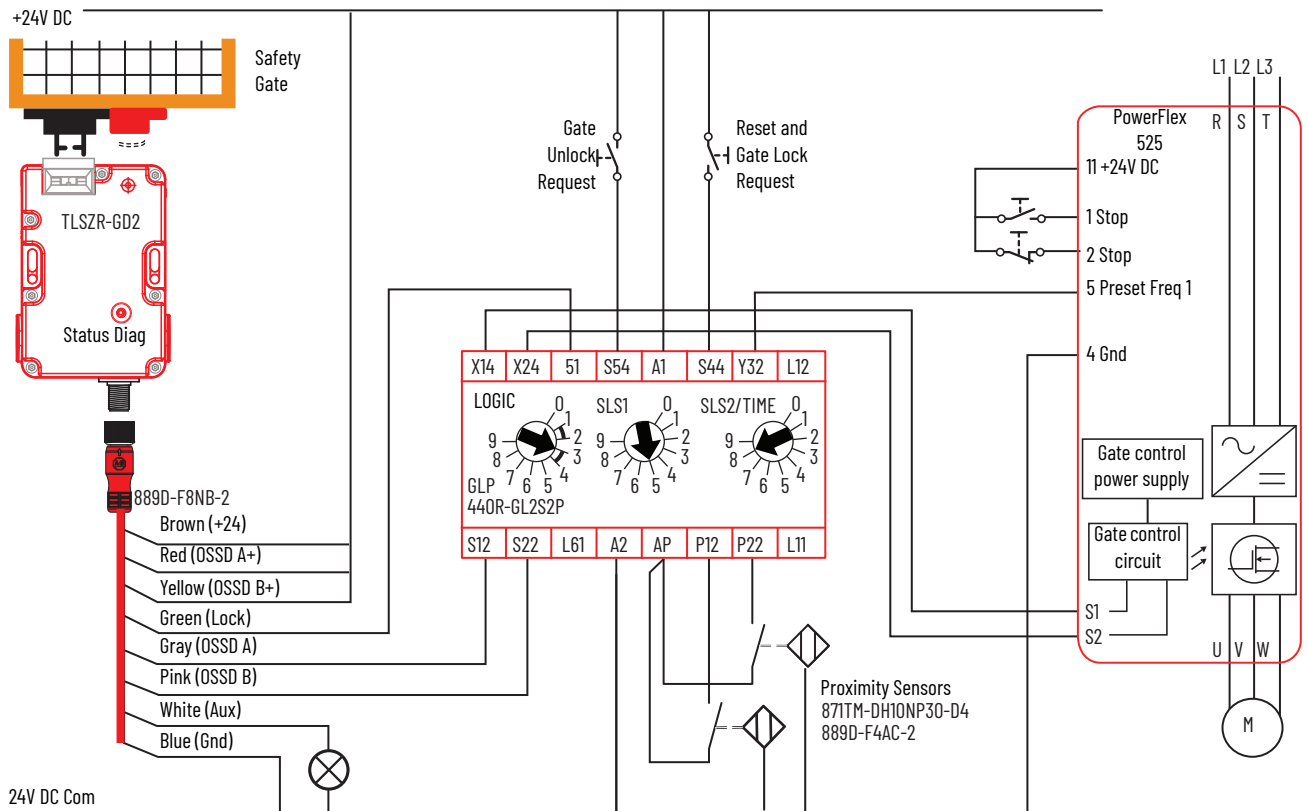
Figure 16 - GLP and TLSZR Schematic
