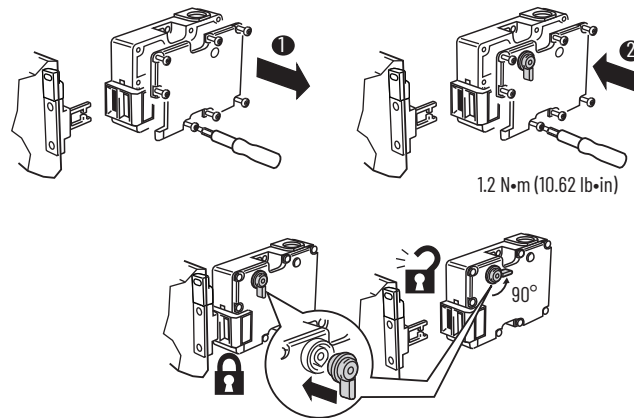
Figure 7 - Manual Override Cover
