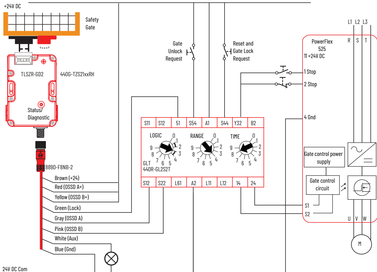
Figure 17 - GLT and TLSZR Schematic
