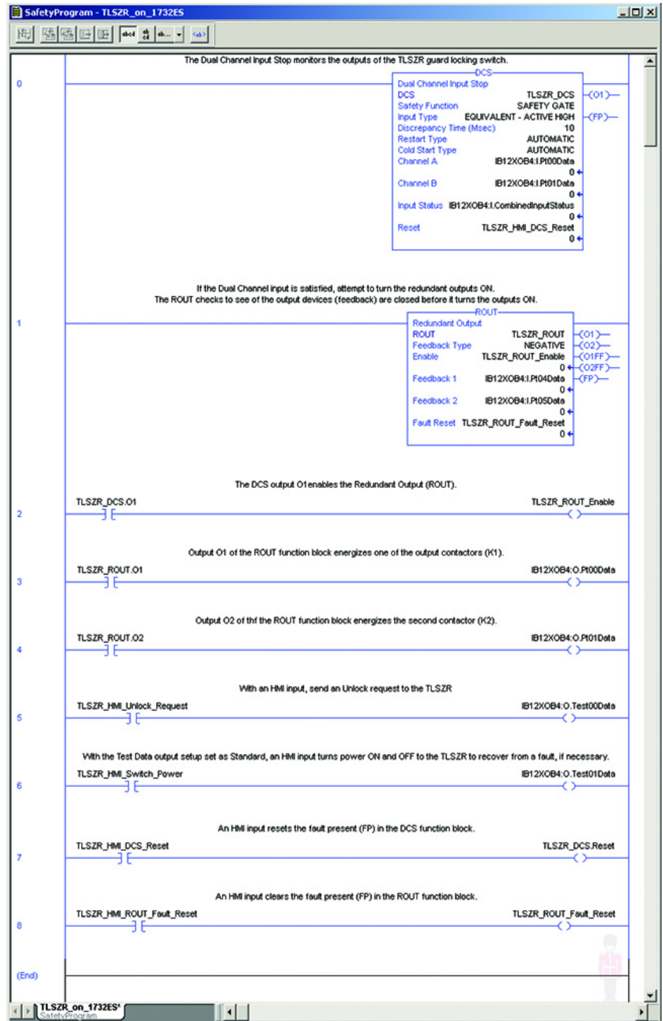
Figure 34 - Example Studio 5000 Program
