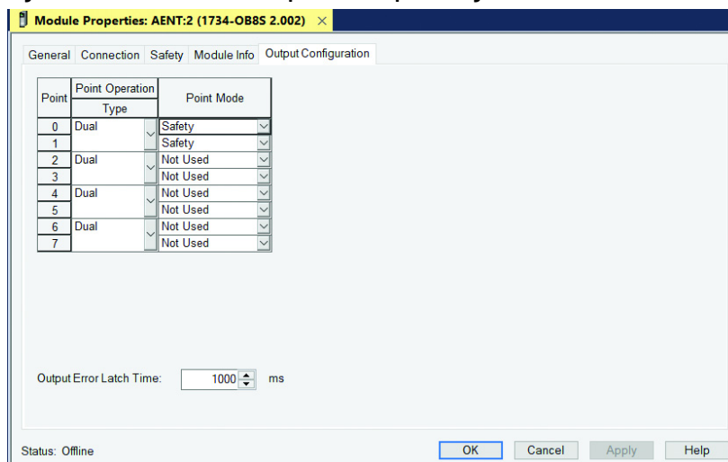
Figure 27 - 1734-OB8S Module Properties - Output Configuration
