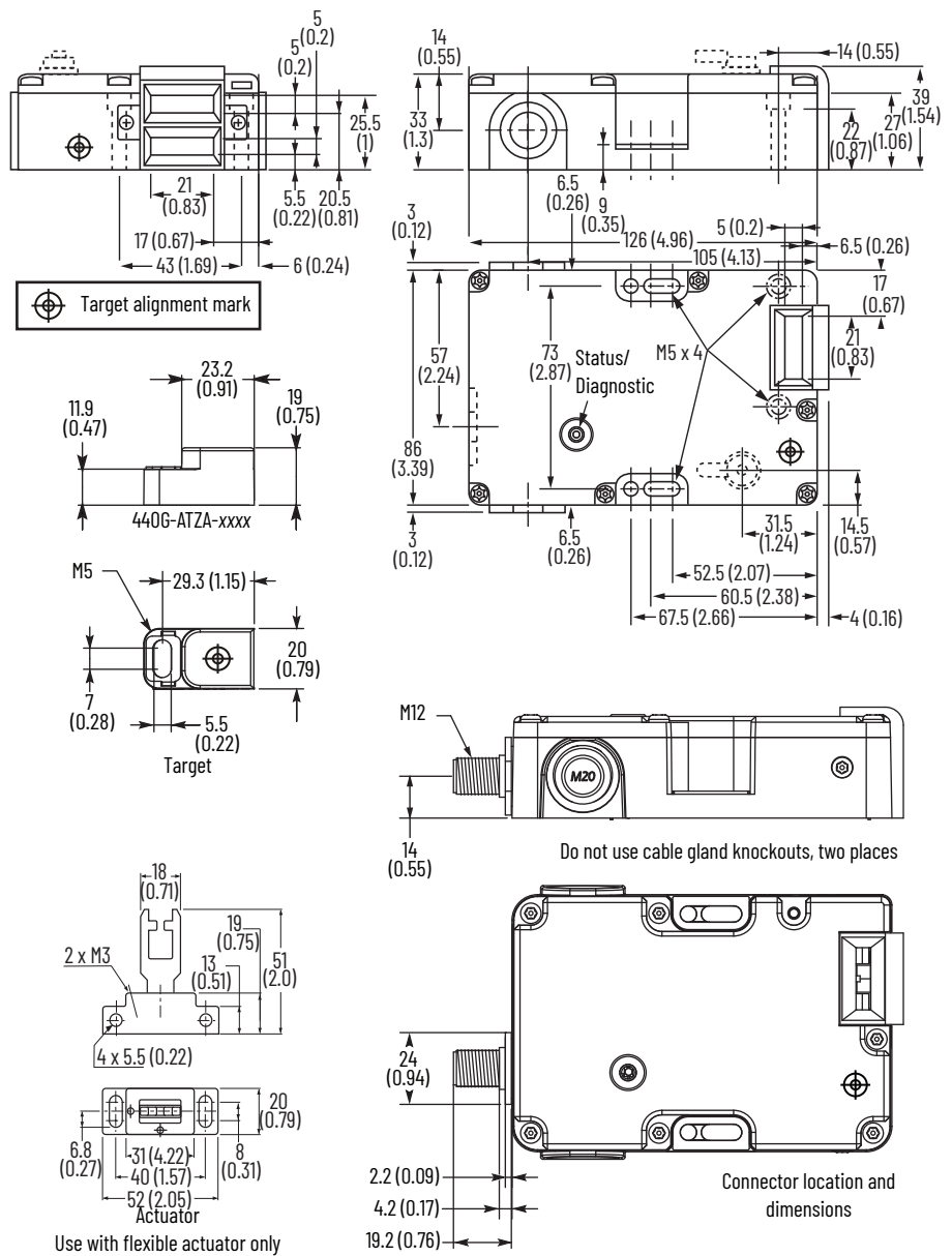
Figure 12 - Approximate Dimensions [ mm (in.) ]
