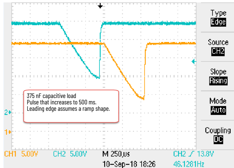
Figure 41 - Typical Capacitive Effect on Pulse Tests
