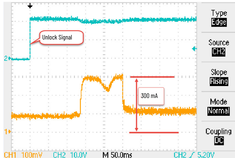
Figure 43 - Inrush Current on the Power Supply at the Guard Locking Switch
