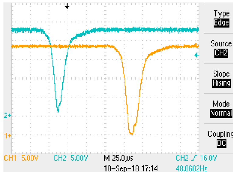
Figure 39 - TLSZ Test Pulses Into a 1K Resistive Load
