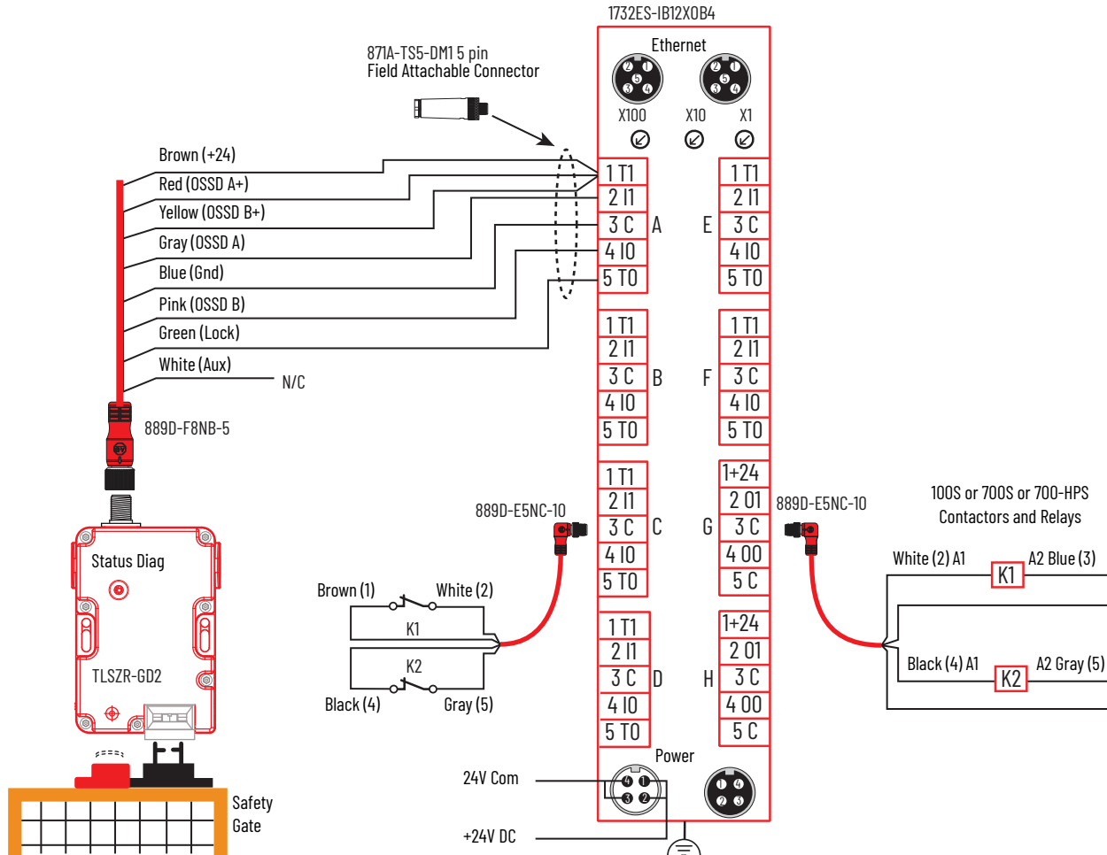
Figure 29 - ArmorBlock Schematic
