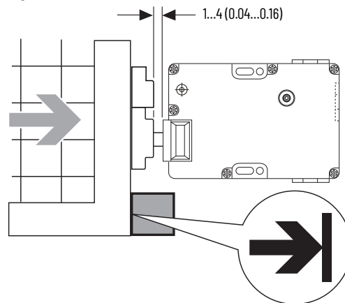
Figure 10 - Clearance and Insertion Distance [mm (in.)]
