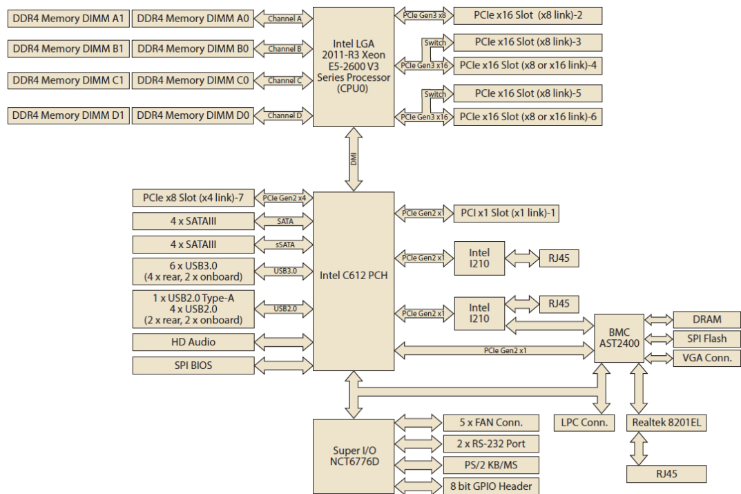
Figure 1.3 Block Diagram
