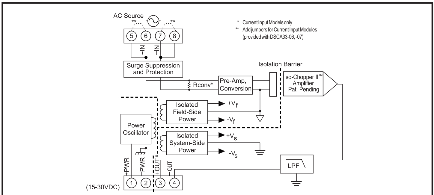
Figure 1: DSCA33 Block Diagram
