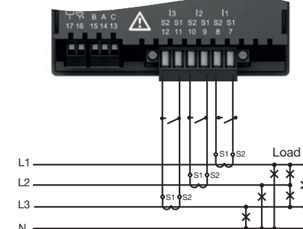
Connection "Current measurement via current transformer"
