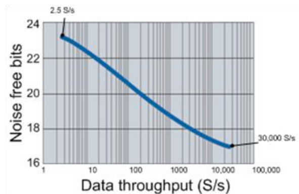
Figure 8. USB-2408 Series A/D converter data rate vs. noise graph
