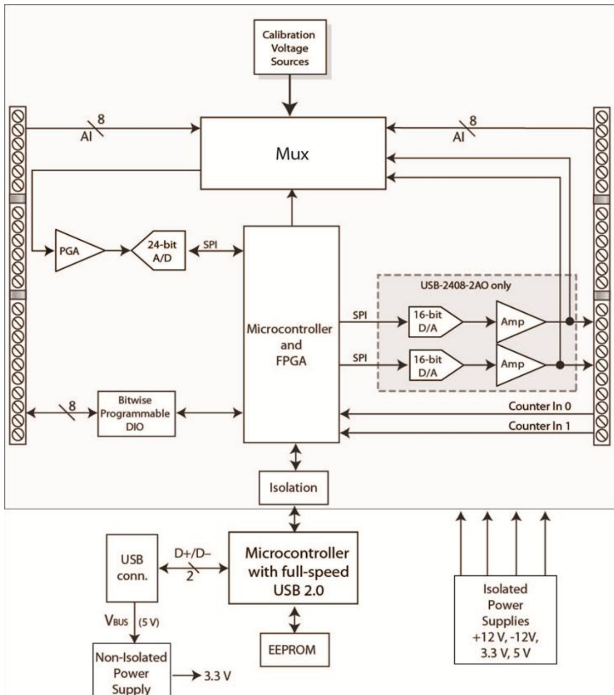
Figure 1. USB-2408 Series functional block diagram
