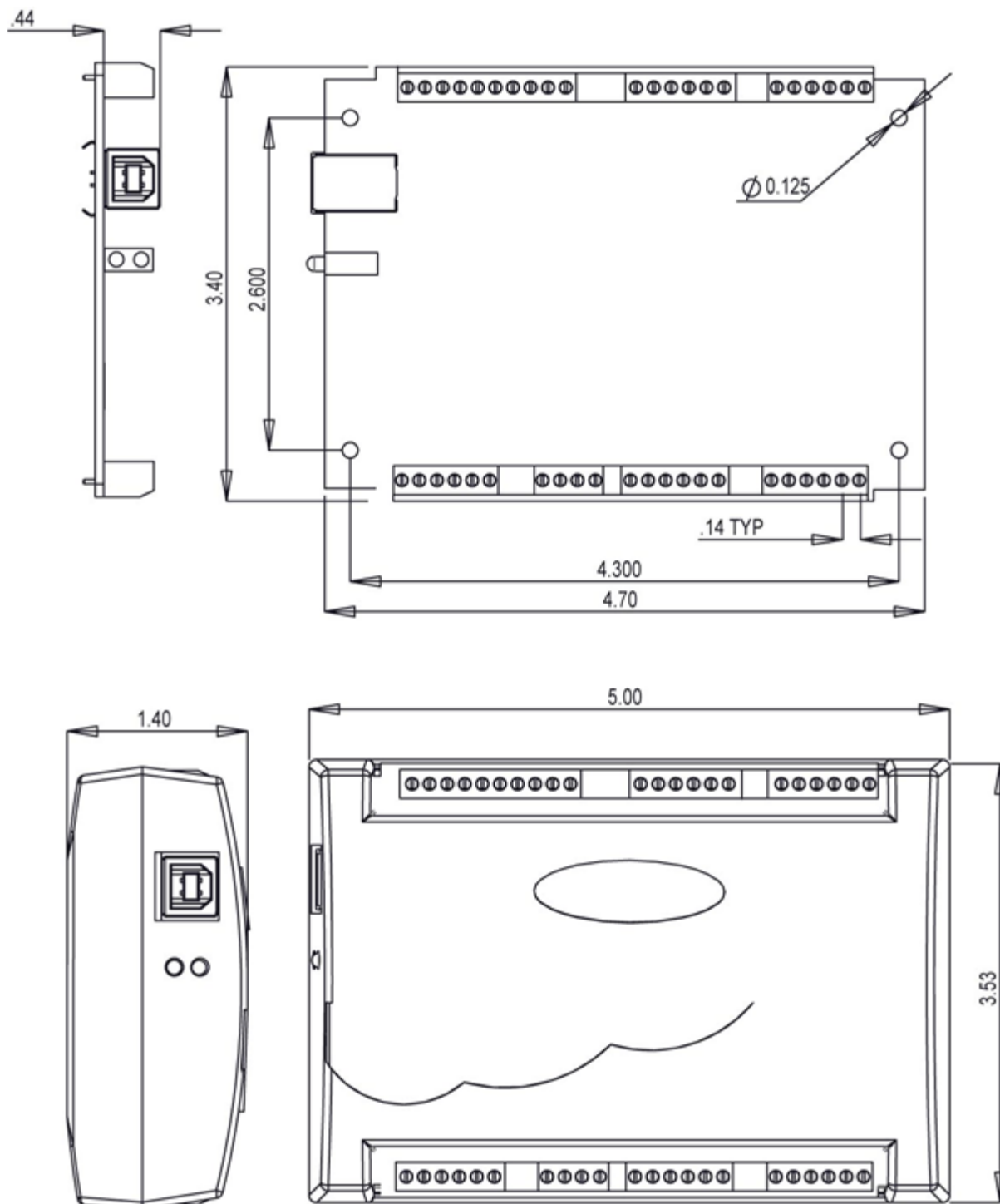
Figure 14. USB-2408 Series device circuit board (top) and enclosure dimensions
