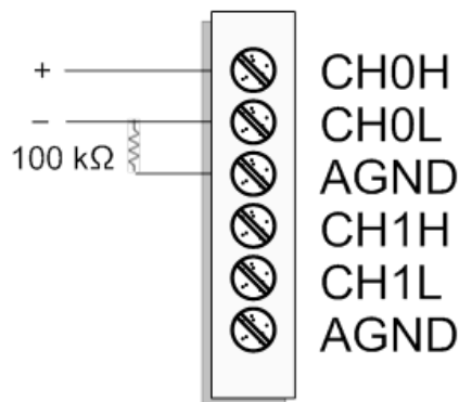
Figure 6. DIFF voltage connection with ground path resistor example
