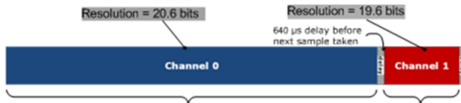
Figure 9. USB-2408 Series data rate vs. resolution example
