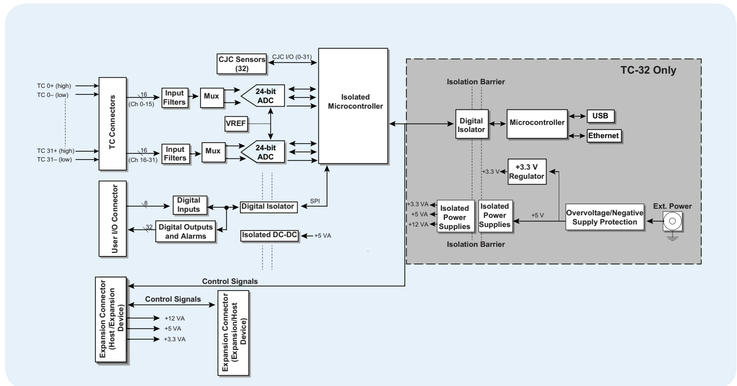
TC-32 and TC-32-EXP Block Diagram
