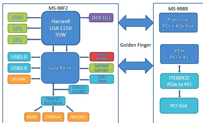
MS-9A66 Block Diagram
