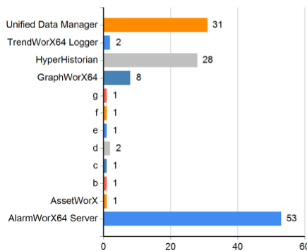
Bad Points Distribution Across Applications
